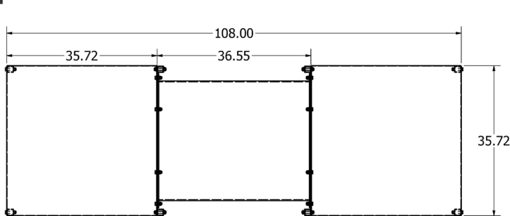
6507 STEP UP TABLE TOP VIEW
